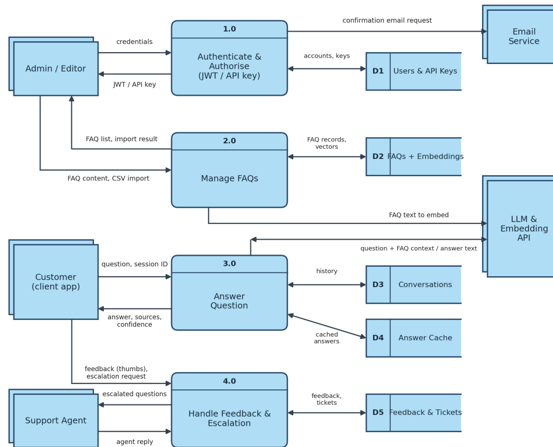
Figure 1: Level-1 Data Flow Diagram of AI FAQ Assistant API
